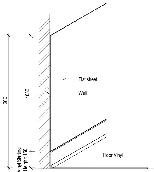
Detail of Flat Sheet with vinyl skirting
