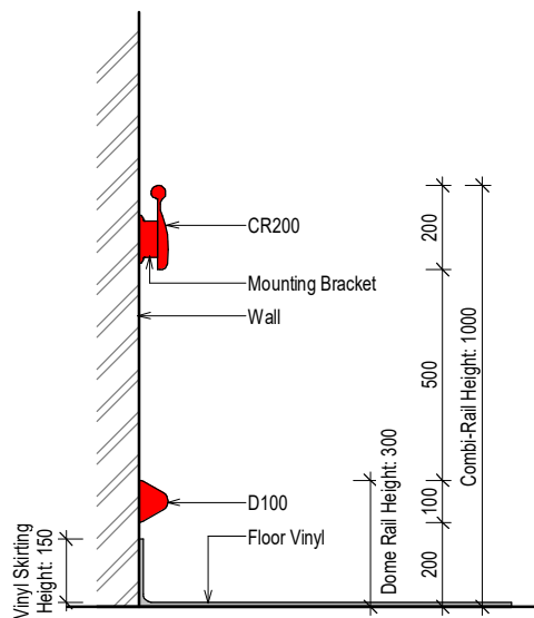
Section Detail with vinyl skirting
