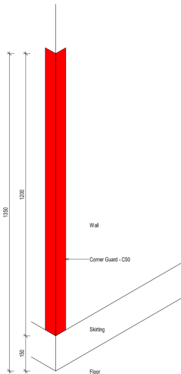
CORNER GUARD - 1200mm HIGH
