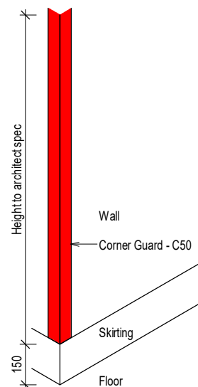
Detail of Corner Guard
